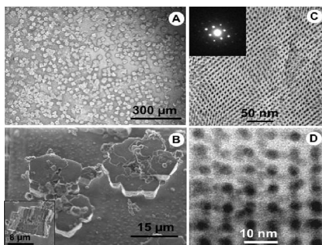
Fig. 6 SEM and TEM images of hierarchical NC mesostructure arrays on glass slides. (A) A low resolution SEM image. (B) A magnified SEM image of (A). Inset shows a cross-sectional image. Representative TEM images from (C) [110] orientation and (D) [100] orientation. The inset of (C) shows the selected area electron diffraction pattern from the image in (C). Adapted from ref. 48.
